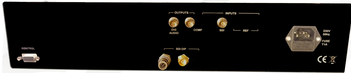
Rear View of Standard Version Back Panel
